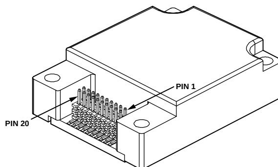
Figure 6. Pin Locations
