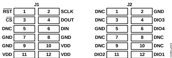
Figure 23. J1/J2 Pin Assignments for Interface PCB
