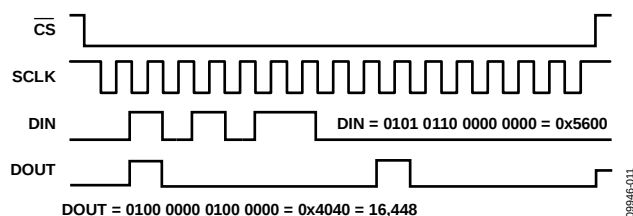
Figure 14. SPI Test Read Pattern DIN = 0x5600, DOUT = 0x4040
