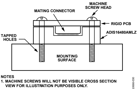
Figure 32. Cross-Section View of Rigid PCB for the Mating Connector
