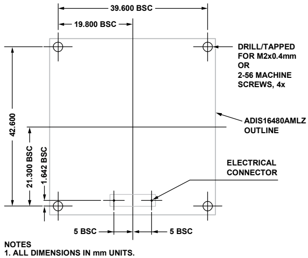
Figure 31. Suggested Hole Locations, Connector-up
