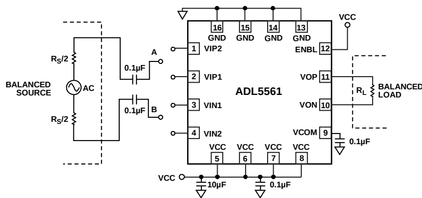
Figure 33. Basic Connections
