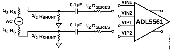
Figure 38. Gain Adjustment Using Series Resistor
