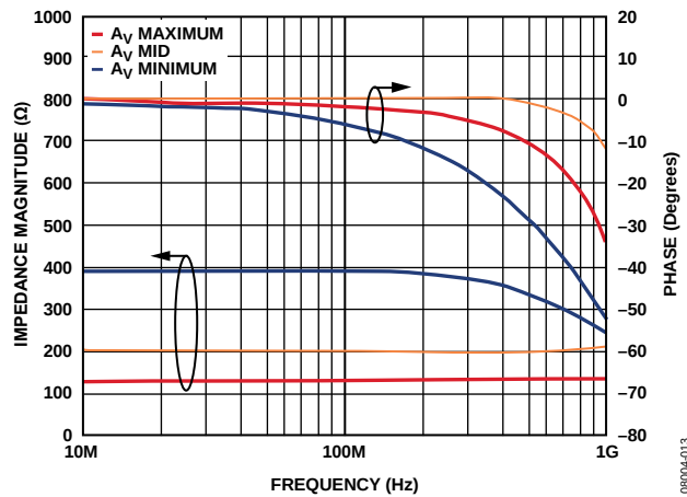
Figure 28. Input Impedance Magnitude and Phase vs. Frequency
