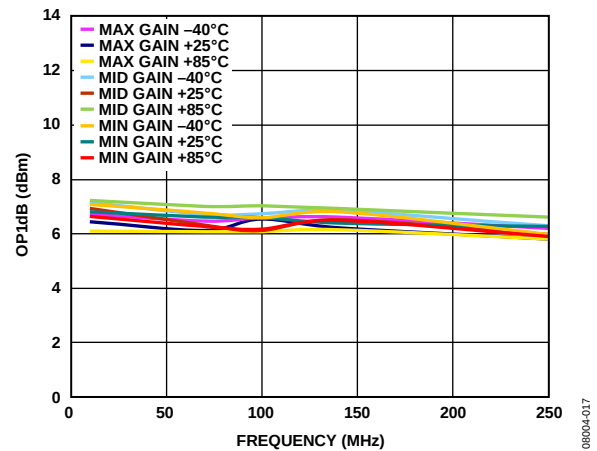
Figure 7. Output P1dB (OP1dB) vs. Frequency at A_V = 6\text{ dB} , A_V = 12\text{ dB} , and A_V = 15.5\text{ dB} over Temperature, 1\text{ k}\Omega Differential Load
