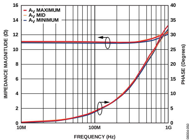
Figure 29. Output Impedance Magnitude and Phase vs. Frequency
