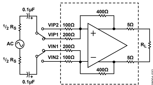
Figure 32. Basic Structure
