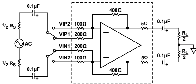
Figure 35. Differential Input Loading Circuit
