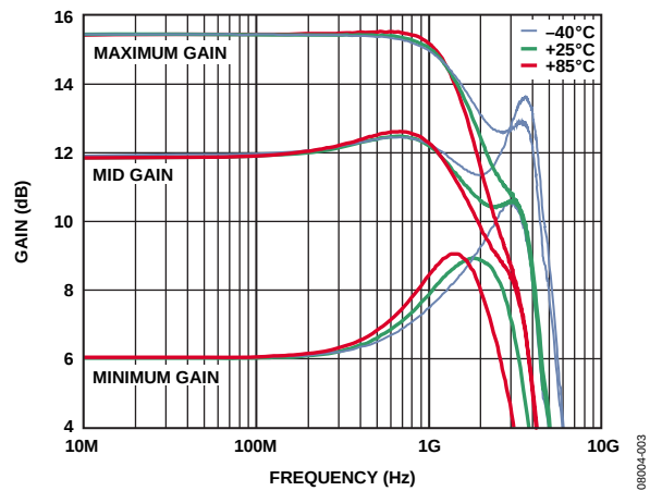
Figure 4. Gain vs. Frequency Response for 1\text{ k}\Omega Differential Load, A_V = 6\text{ dB} , A_V = 12\text{ dB} , and A_V = 15.5\text{ dB} over Temperature
