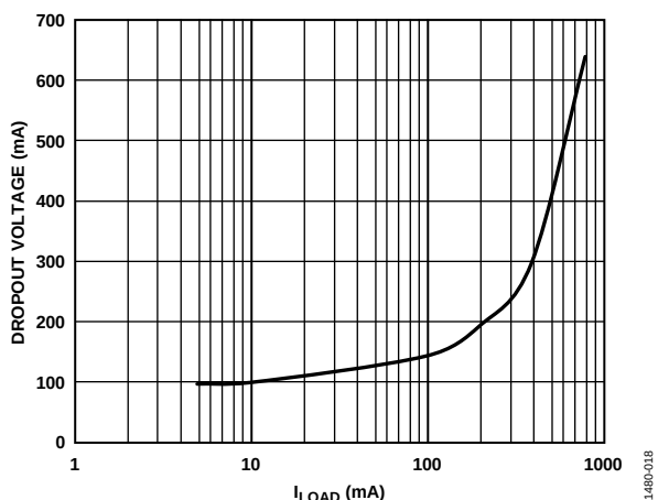
Figure 18. Dropout Voltage vs. Load Current ( I_{LOAD} ), ADM7151-04, V_{OUT} = 5 V
