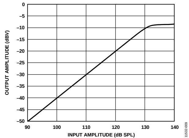
Figure 9. Linearity
