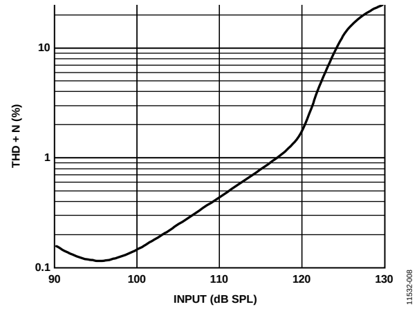
Figure 8. THD + N vs. Input SPL
