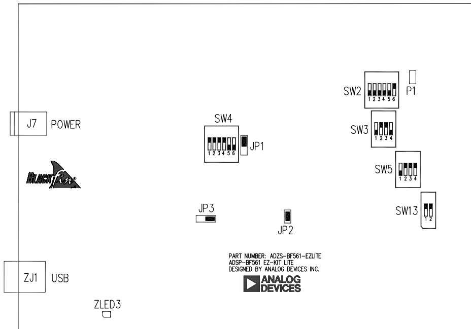
Figure 1-1. EZ-KIT Lite Hardware Setup
