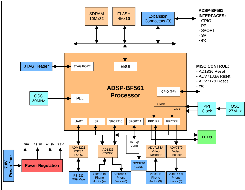
Figure 2-1. System Architecture
