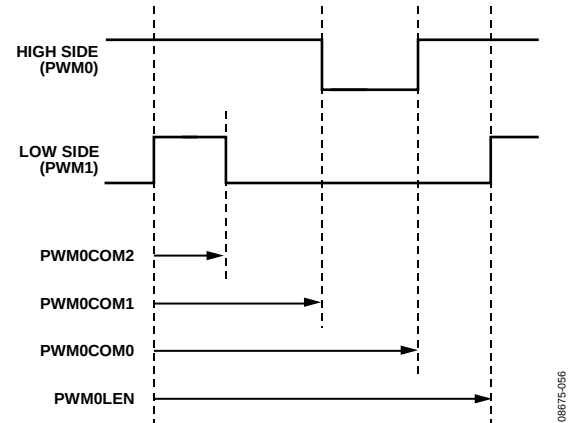
Figure 40. PWM Timing
