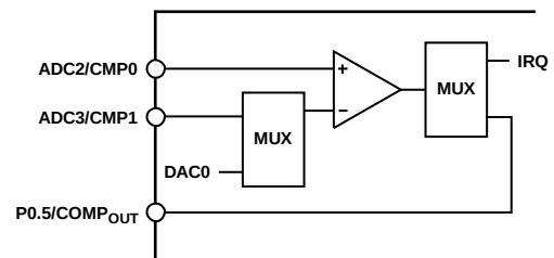
Figure 34. Comparator
