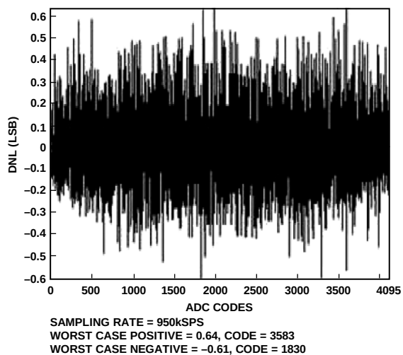
Figure 12. Typical DNL, f_{ADC} = 950 kSPS, External 1.0 V Reference Used
