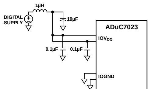
Figure 48. Recommended IOV_{DD} Supply Filter
