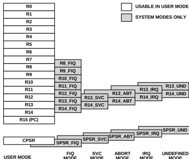
Figure 15. Register Organization
