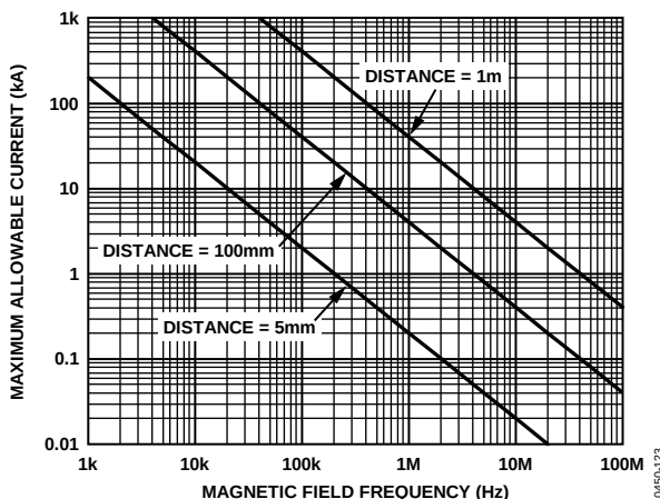
Figure 24. Maximum Allowable Current for Various Current-to- ADuM3223/ADuM4223 Spacings
