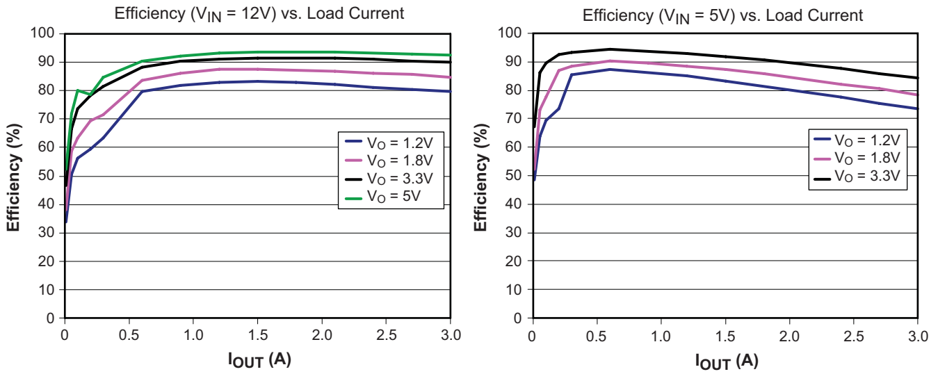
AOZ1031AI Efficiency
