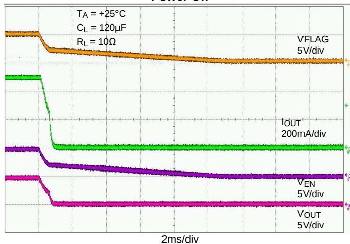
Power Off
