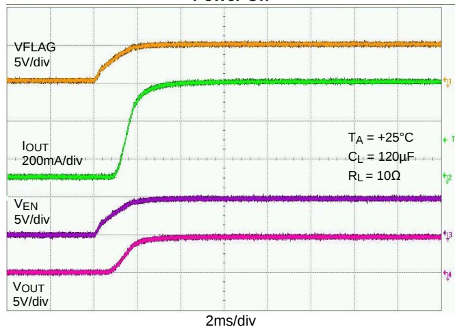
Power On
