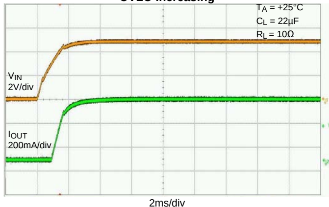
UVLO Increasing
