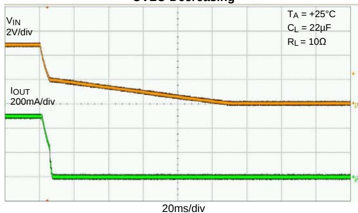
UVLO Decreasing
