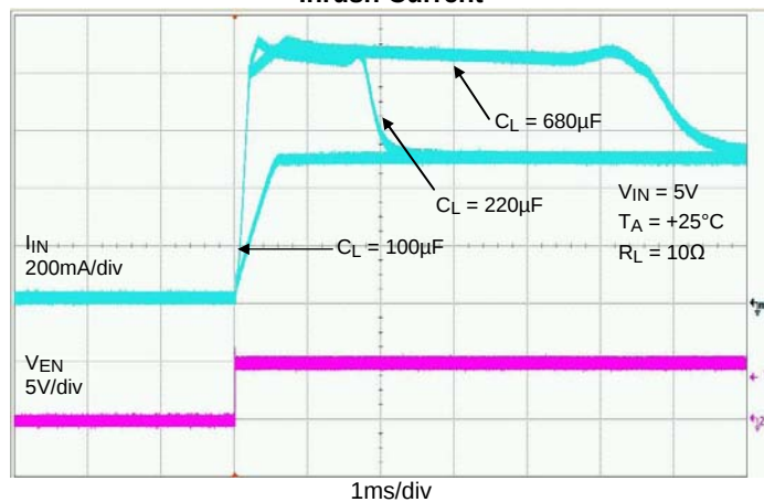
Inrush Current
