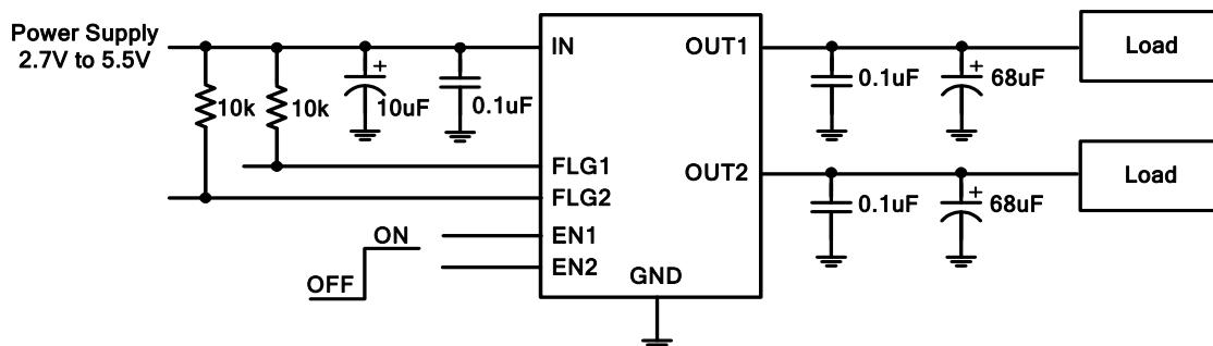
AP2192 Enable Active High
