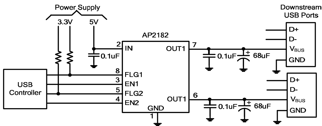
Figure 2 Typical Two-Port USB Host / Self-Powered Hub
