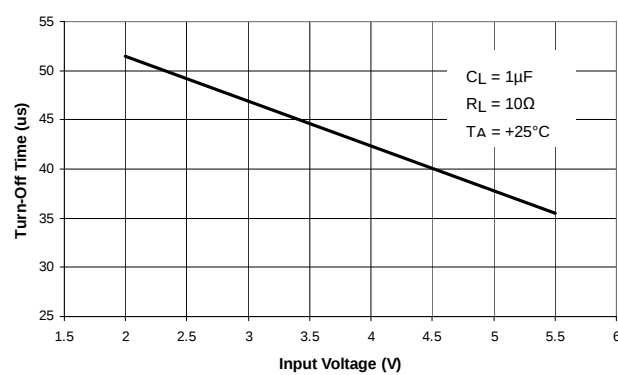
Turn-Off Time vs Input Voltage
