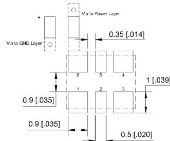
Recommended Land Pattern for LVPECL, LVDS, HCSL
