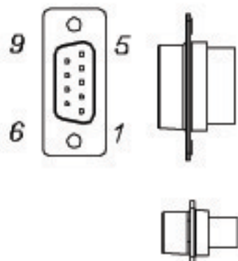
DB9 FEMALE CRIMP TYPE
