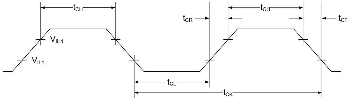
Figure 36-24. External clock drive waveform
