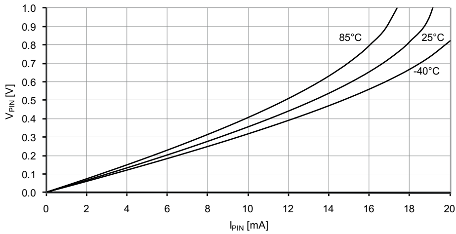
Figure 37-27. I/O pin output voltage vs. sink current.
