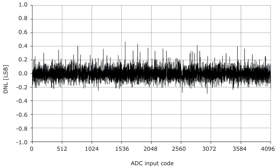
Figure 37-123. DNL error vs. input code.
