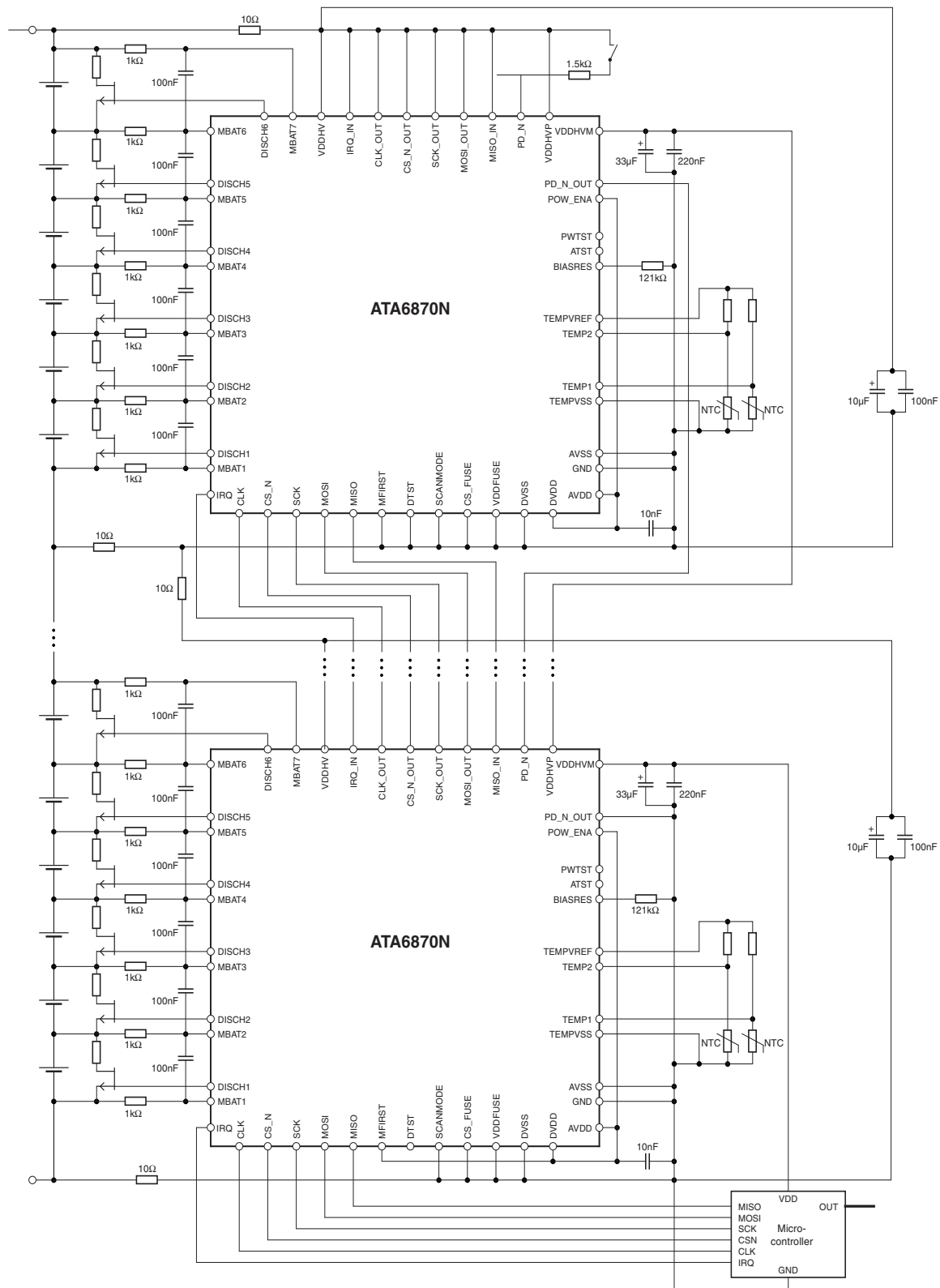
Figure 7-31 shows an application with 2 stacked Atmel® ATA6870Ns.
