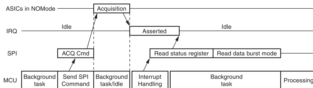
Figure 7-2. Atmel ATA6870N in NORM Mode
