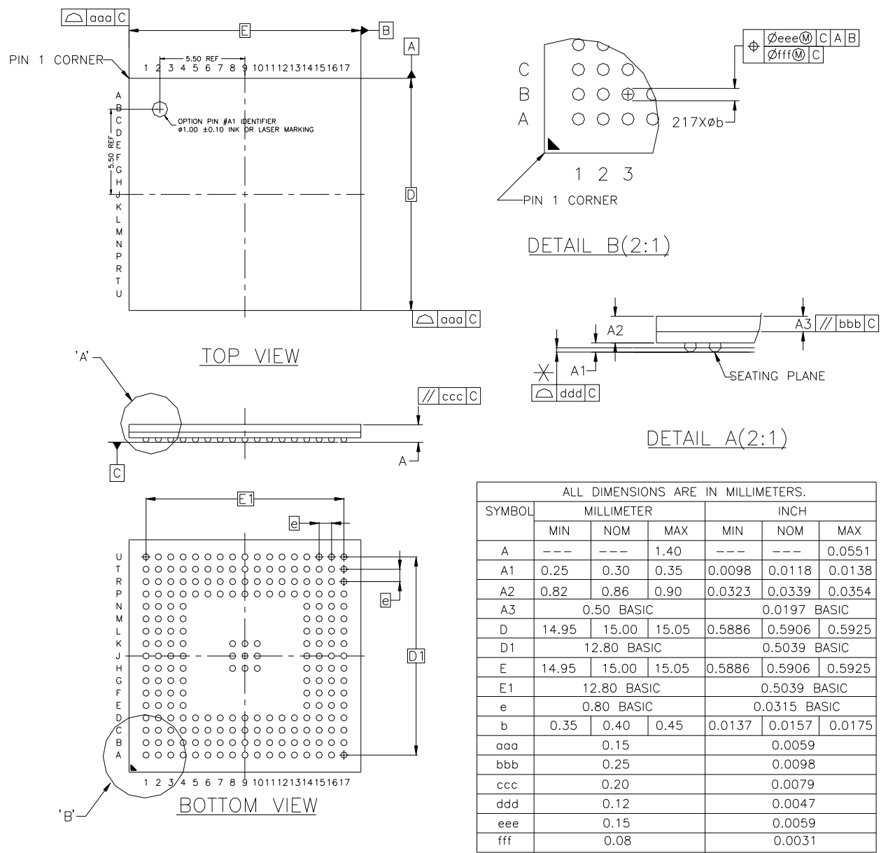
Figure 5-1. 217-ball BGA Package Drawing
