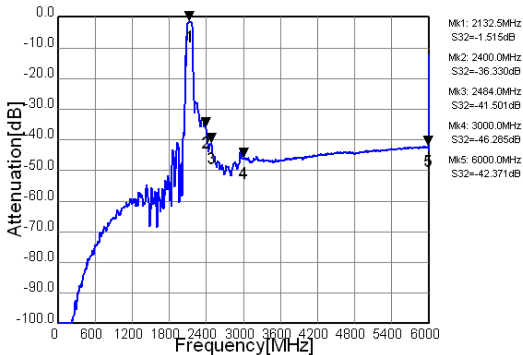
Figure 3-7. Electrical Characteristics
