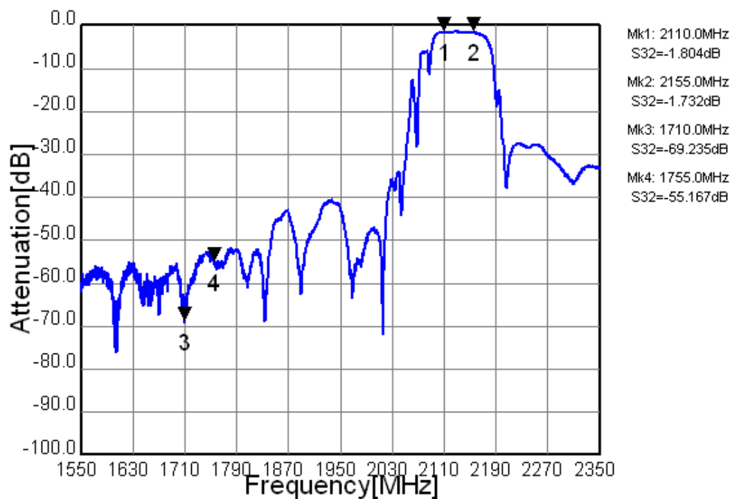
Figure 3-1. Electrical Characteristics
