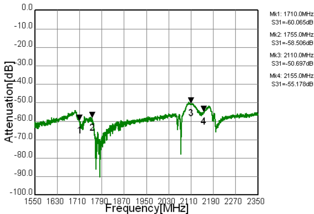
Figure 3-2. Electrical Characteristics
