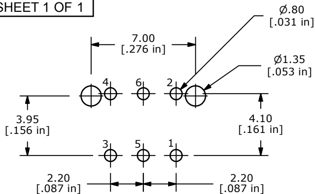
PCB MOUNTING
