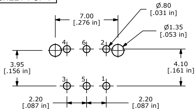
PCB MOUNTING
