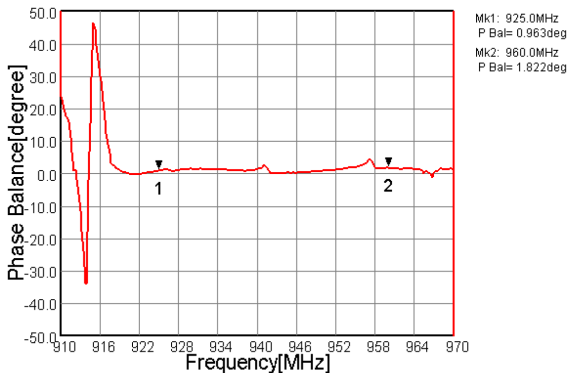
Fig.8 Phase Balance
