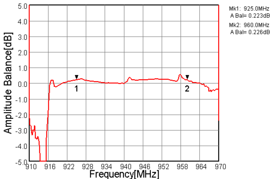
Fig.7 Amplitude Balance
