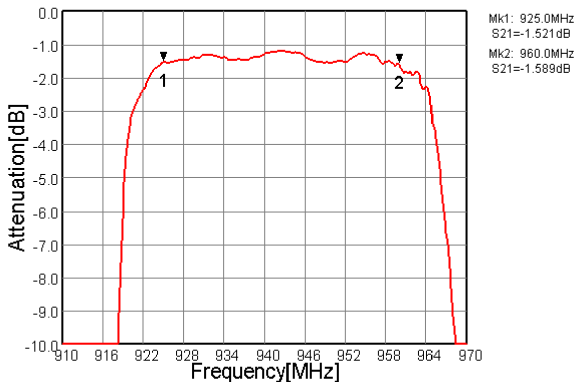
Fig.3 In-band Characteristics
