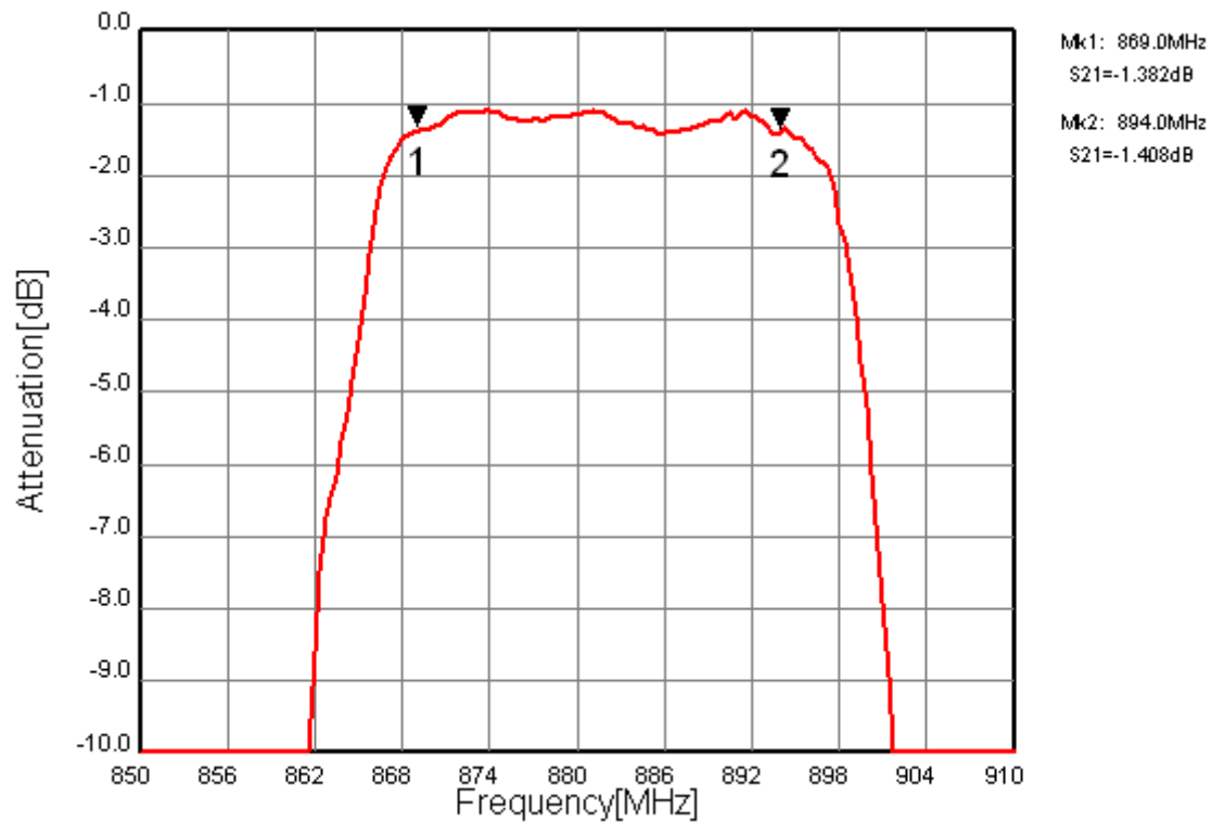
Fig.3 In-band Characteristics
