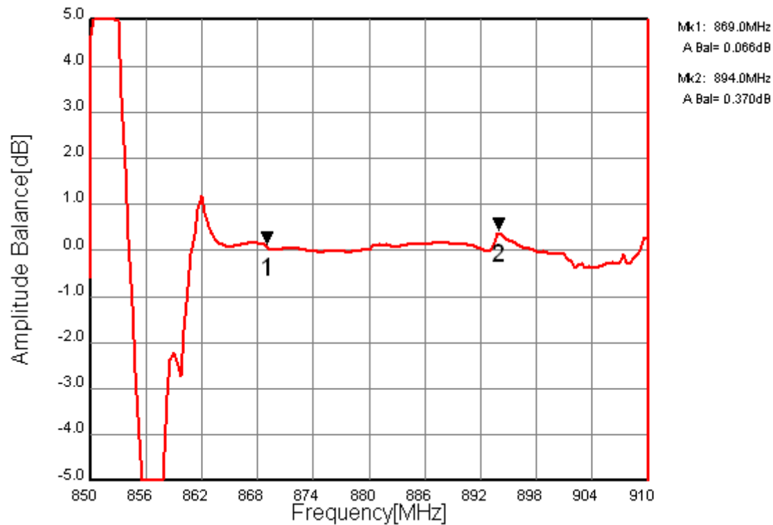
Fig.7 Amplitude Balance
