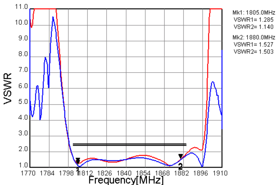
Fig.2 VSWR
