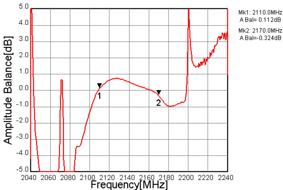
Fig.8 Amplitude Balance
