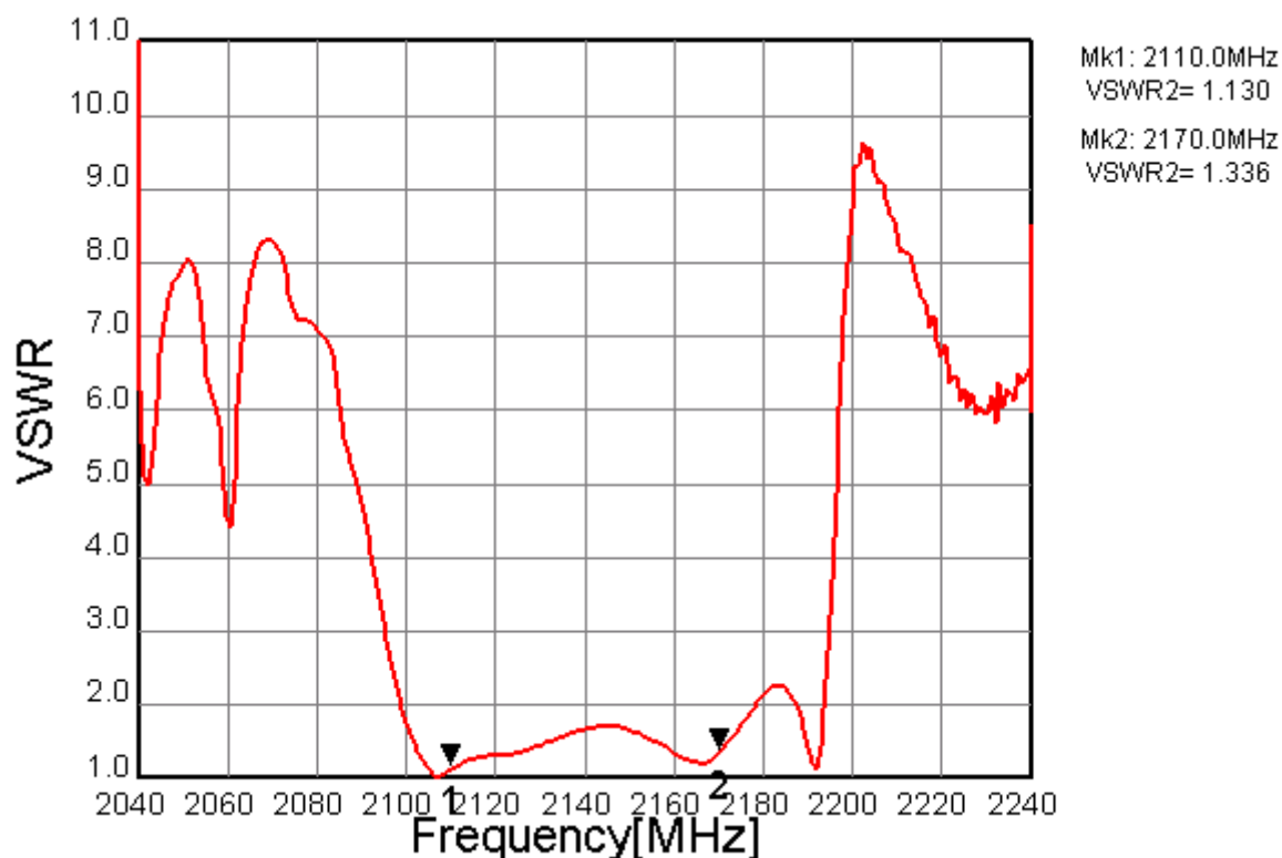
Fig.4 VSWR(bal)
