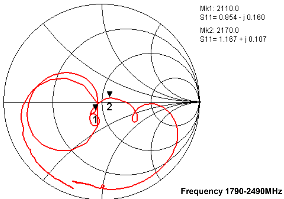
Fig.6 Impedance (unbal)
