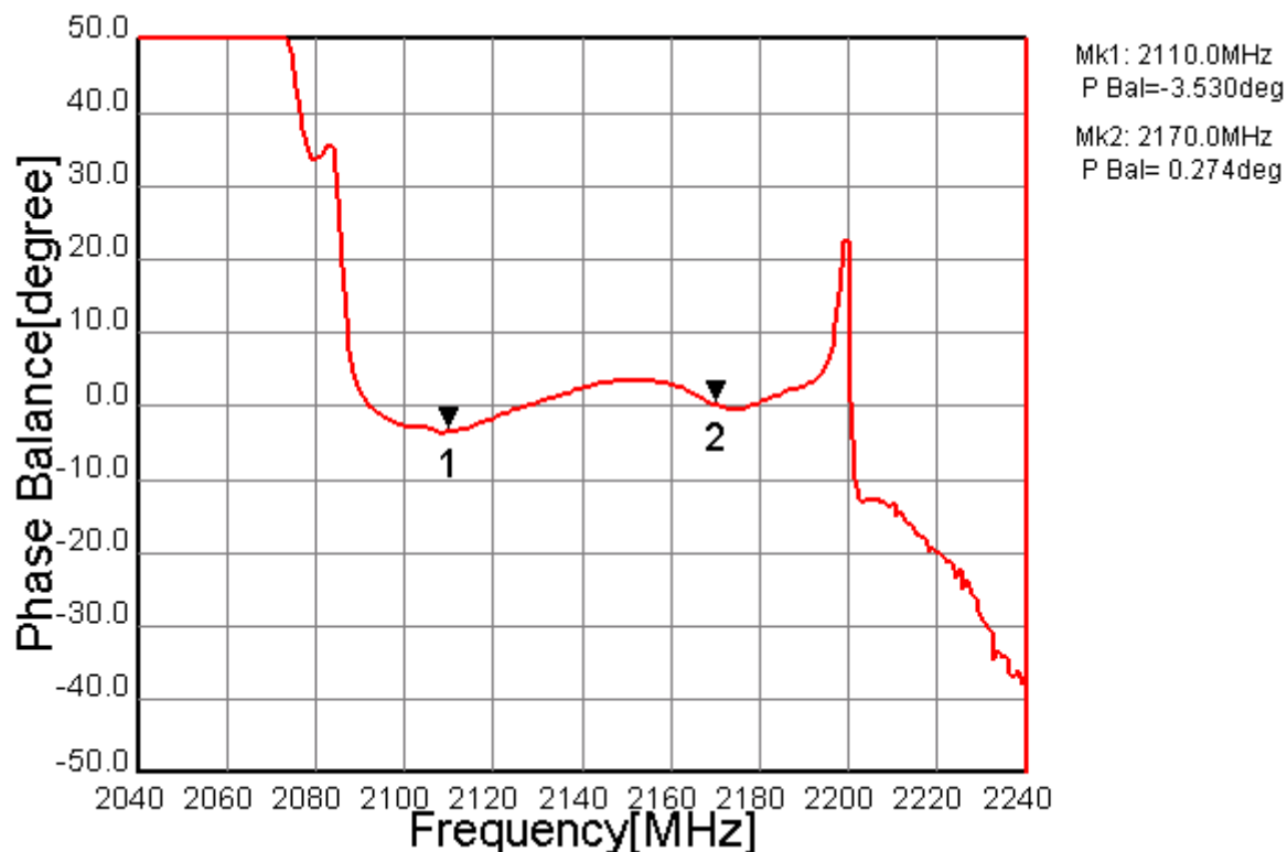
Fig.9 Phase Balance
