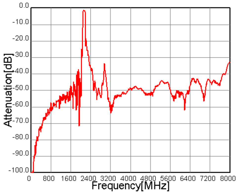
Fig.5 Wide-band Characteristics
