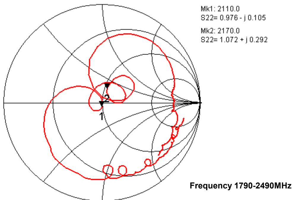
Fig.6 Impedance (unbal)
