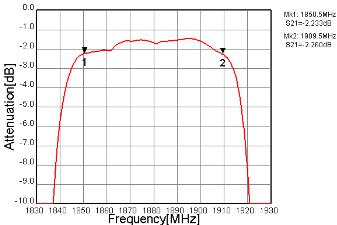
Fig.1-3 In-band Characteristics
