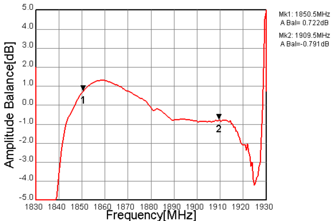
Fig.1-7 Amplitude Balance
