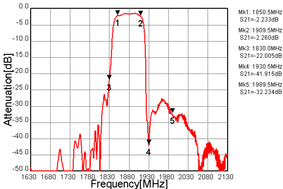
Fig.1-1 Pass-band-Characteristics
