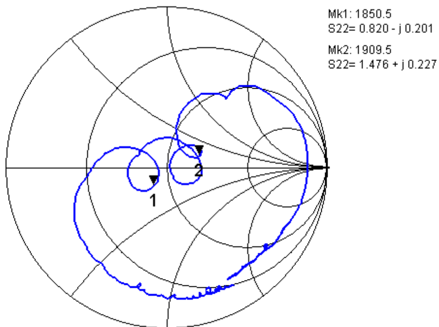
Fig.1-5 Output Impedance (unbalance)
