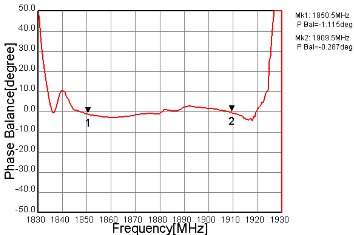
Fig.1-8 Phase Balance
