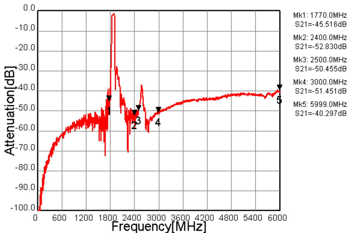
Fig.1-4 Wide-band Characteristics
