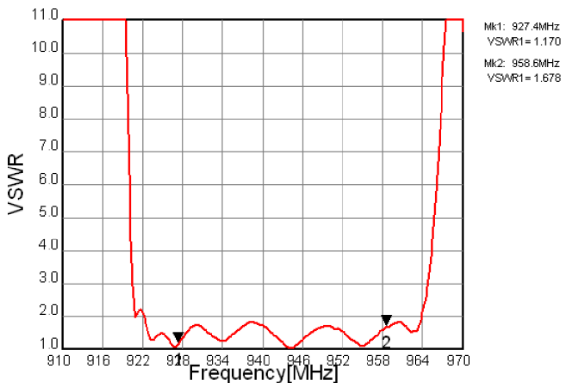
Fig.3 VSWR (INPUT)
