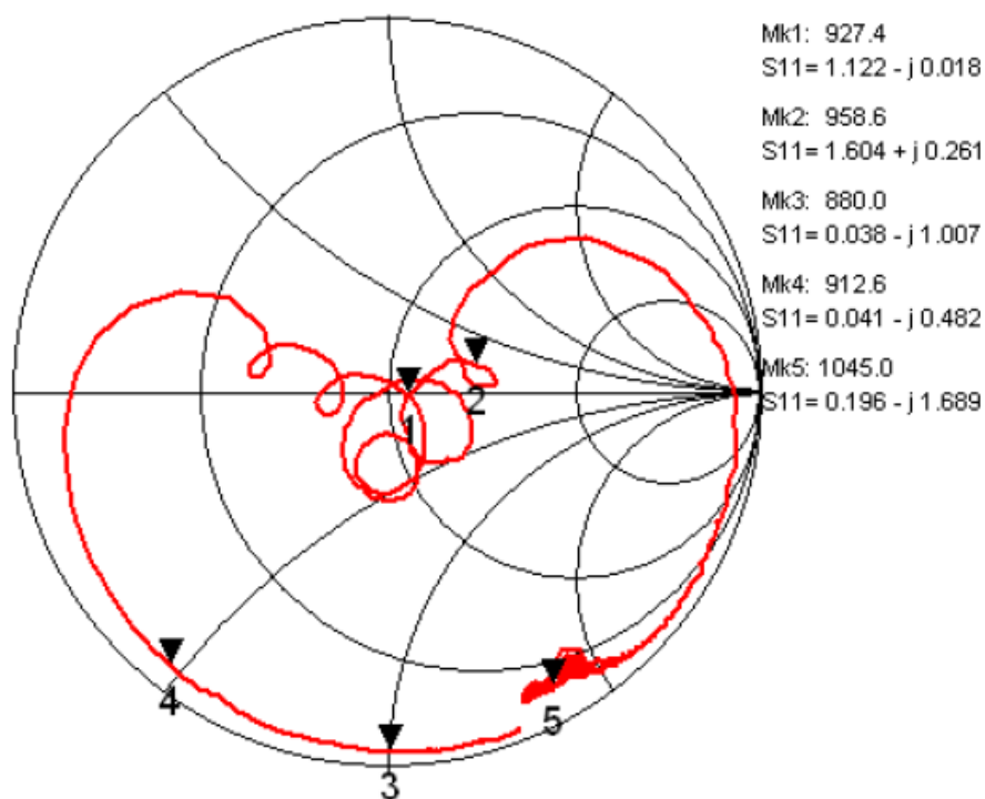
Fig.6 Impedance (Input)
