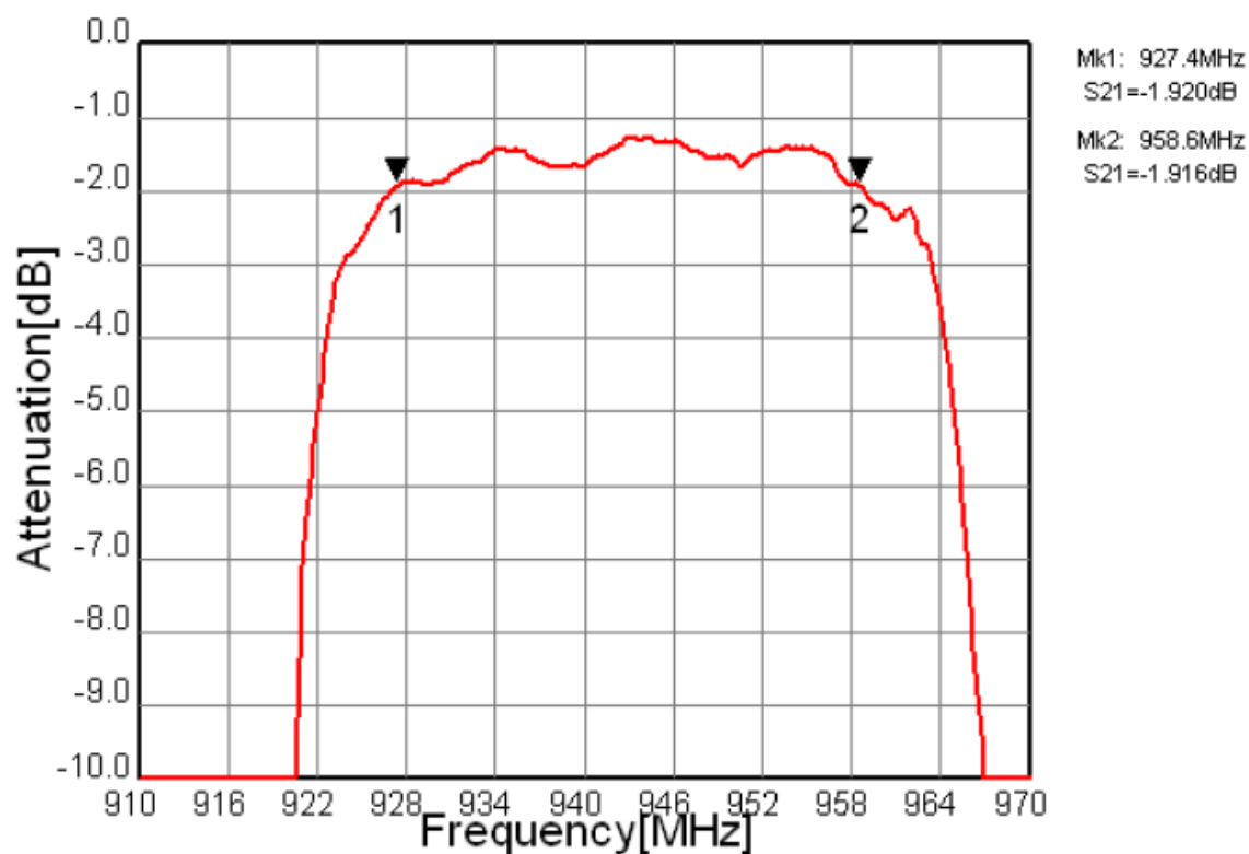
Fig.2 In-band Characteristic
