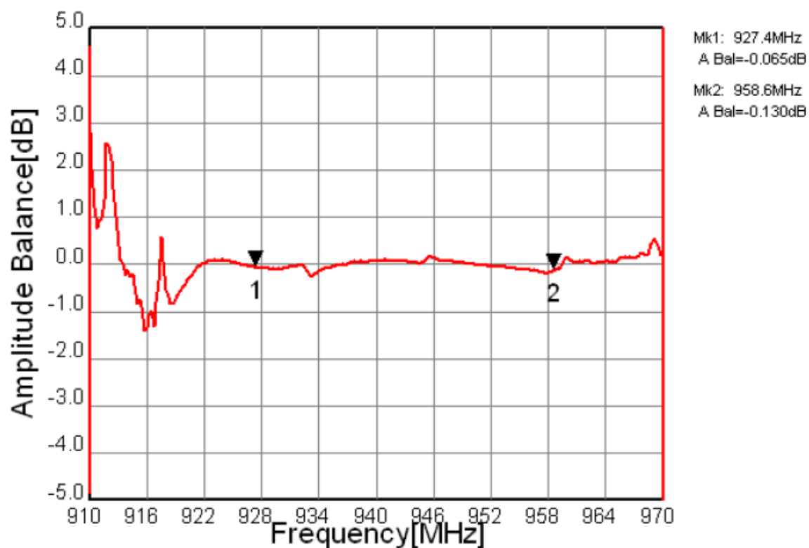
Fig.8 Amplitude balance
