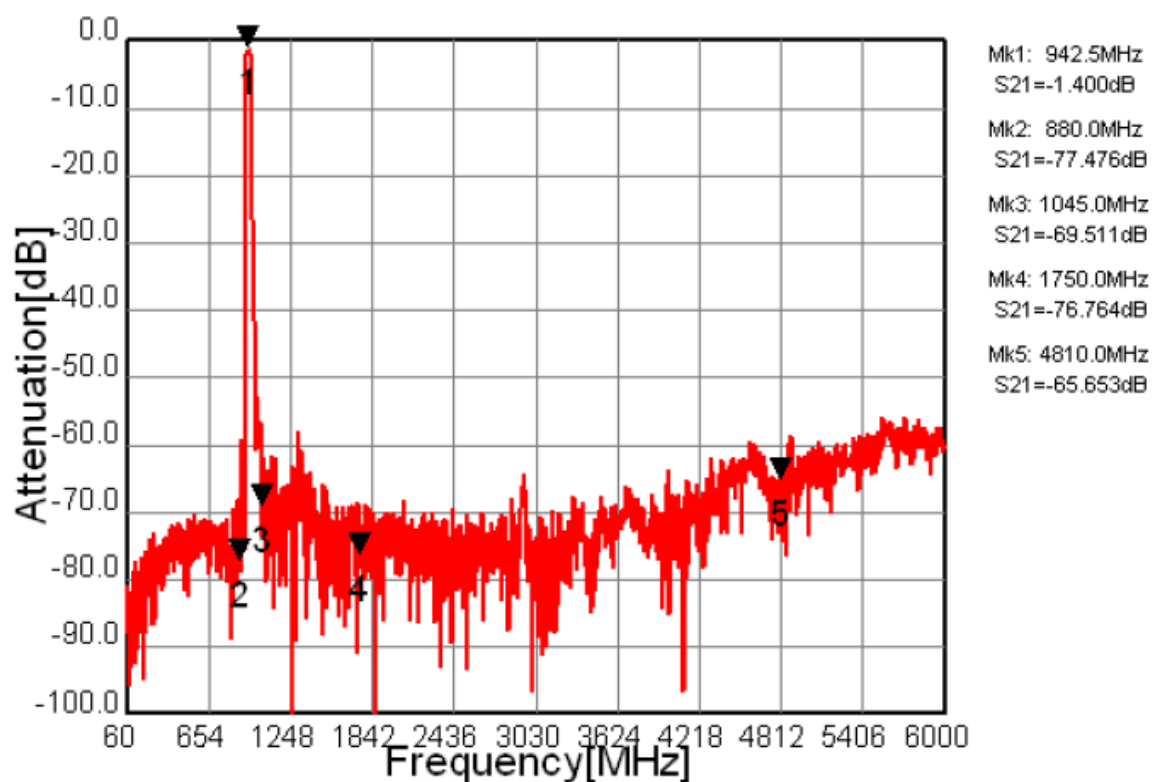
Fig.5 Wide-band Characteristic
