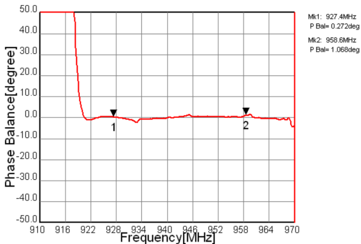
Fig.9 Phase balance
