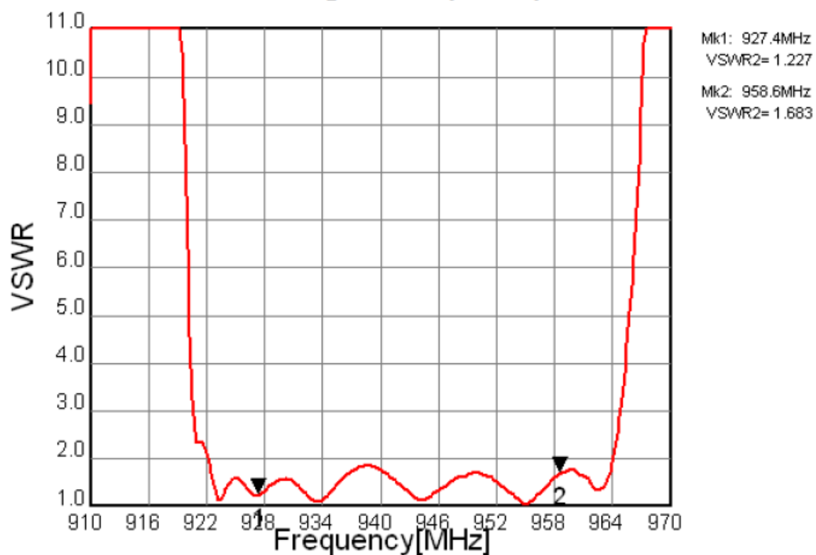
Fig.4 VSWR (OUTPUT)
