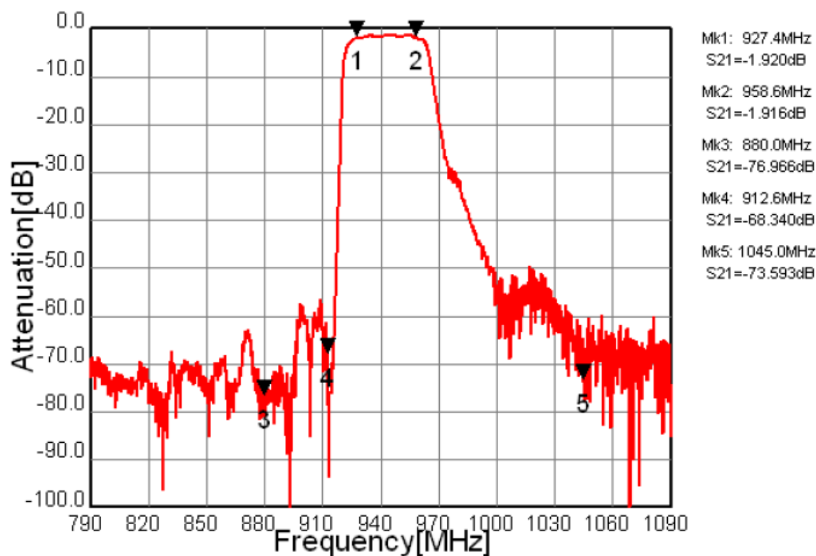
Fig.1 Pass-band Characteristic
