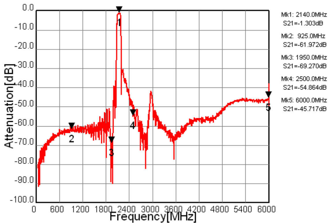
Fig.5 Wide-band Characteristic
