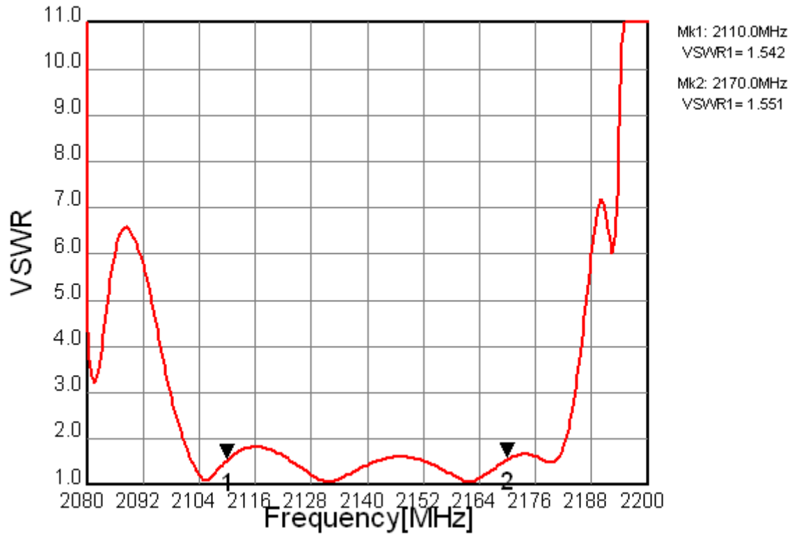
Fig.3 VSWR (INPUT)
