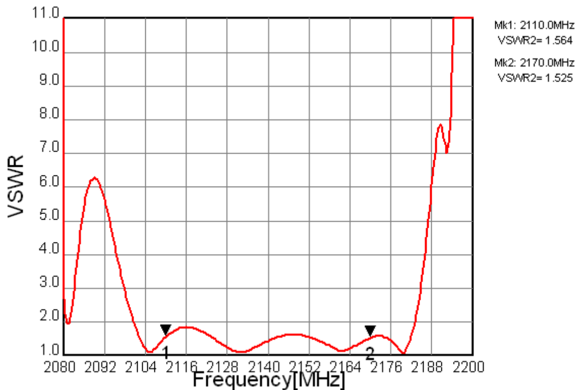
Fig.4 VSWR (OUTPUT)
