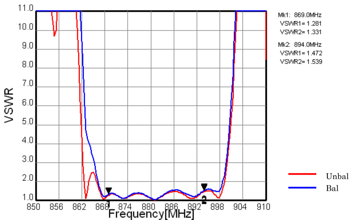
Fig.2 VSWR
