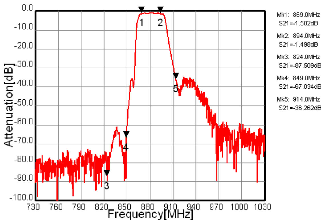
Fig.1 Pass-band Characteristics
