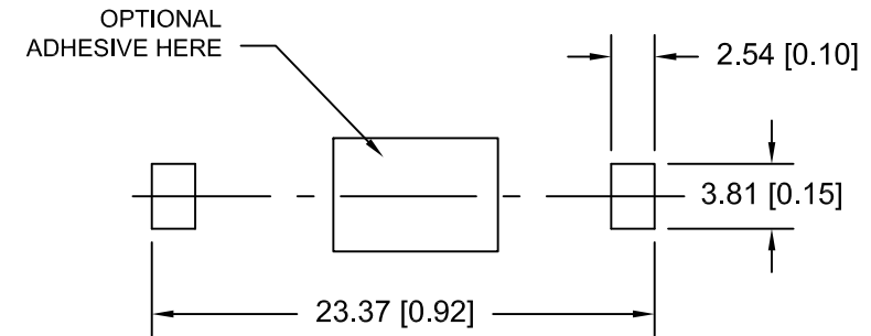
PCB LAYOUT
