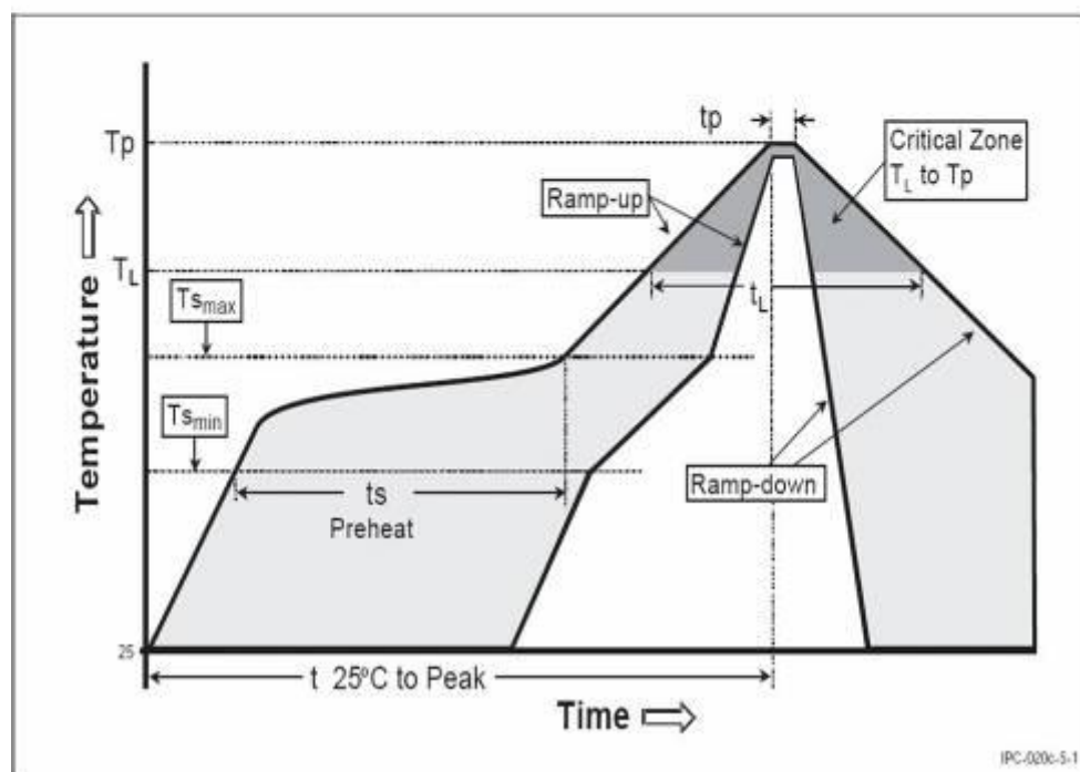
Figure 30: Soldering profile
