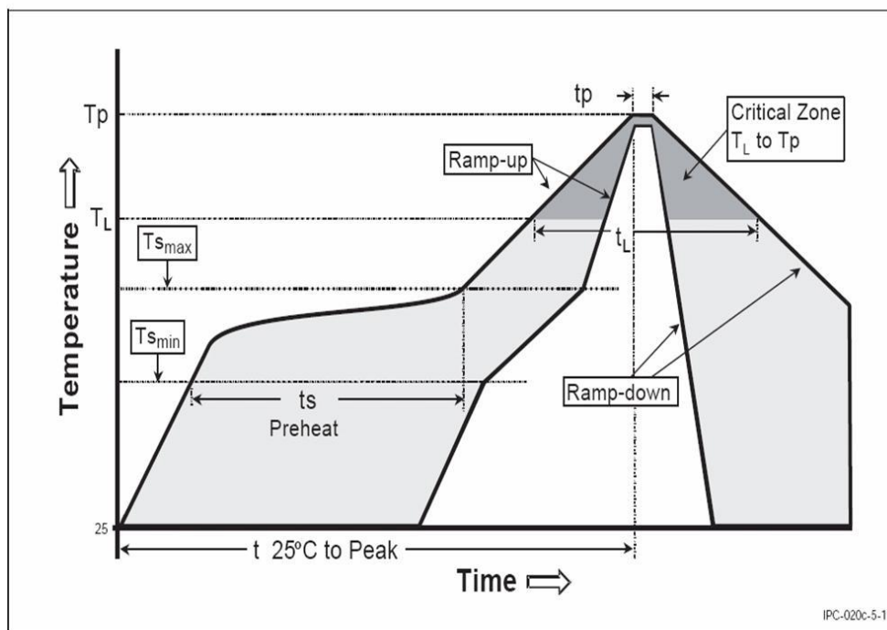
Figure 38: Soldering profile
