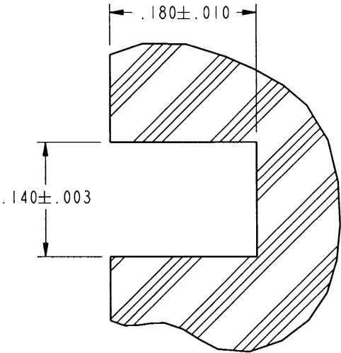
RECOMMENDED PCB CUTOUT SCALE = 6:1
