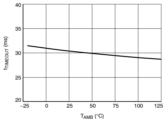
Figure 19. SMBus SCL Clock Low Timeout (Rev. C)
