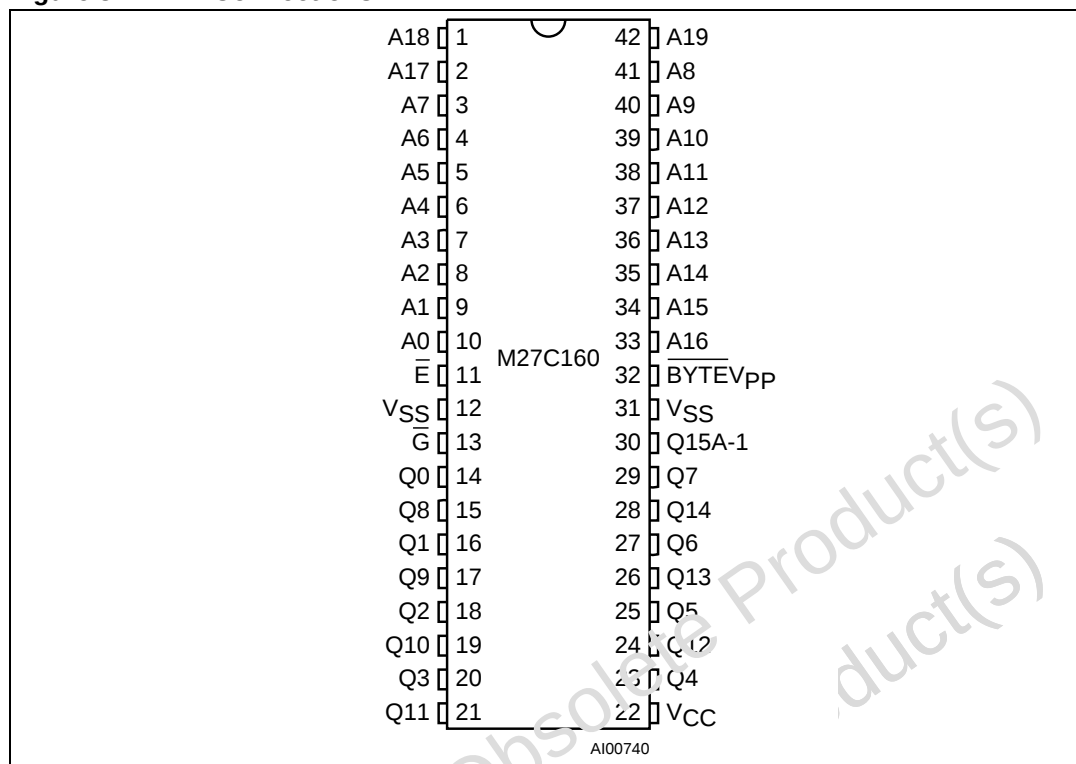
Figure 3. DIP Connections
