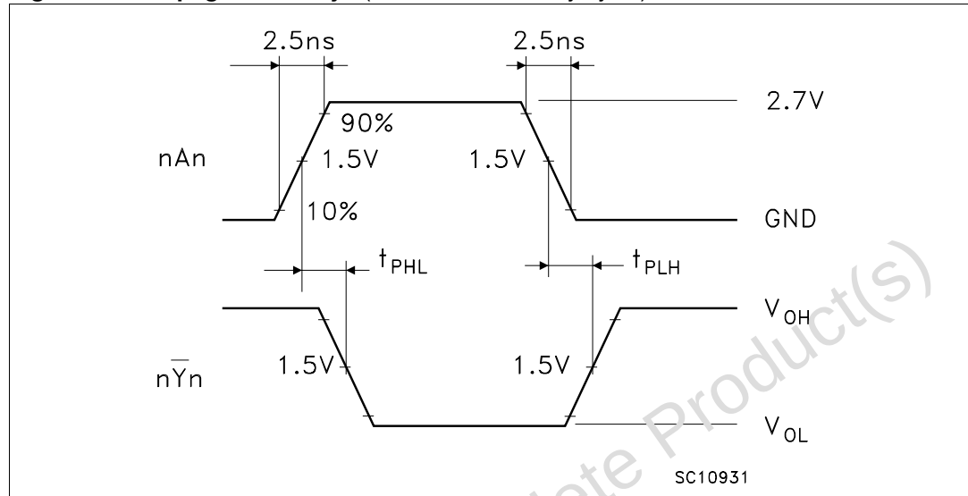
Figure 6. Propagation delays ( f = 1\text{MHz} ; 50% duty cycle)
