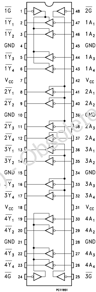
Figure 3. Pin connection (top through view)
