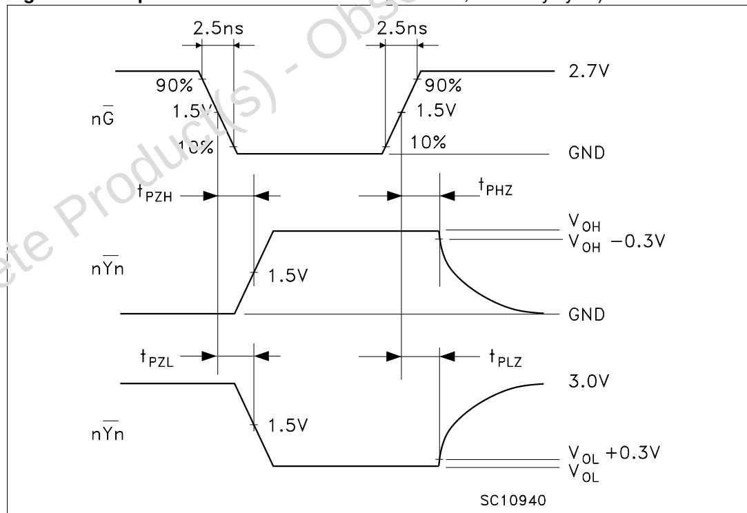
Figure 7. Output enable and disable time ( f = 1\text{MHz} ; 50% duty cycle)
