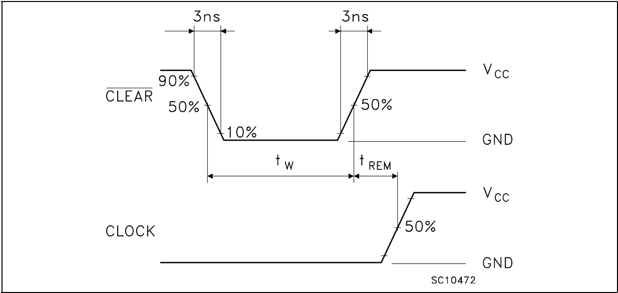
Figure 7: Waveform - Recovery Time (f=1MHz; 50% duty cycle)
