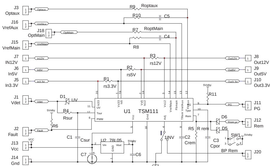
EVALUATION BOARD - ELECTRICAL SCHEMATIC
