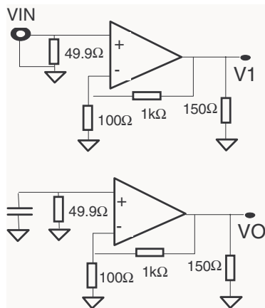
Figure 25. Channel separation (Xtalk) vs. frequency (measurement configuration: Xtalk = 20\log(V0/V1) )
