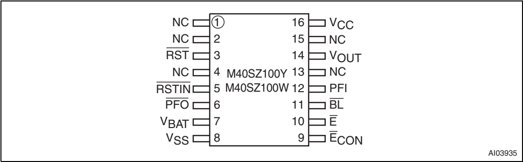
Figure 2. SOIC16 connections
