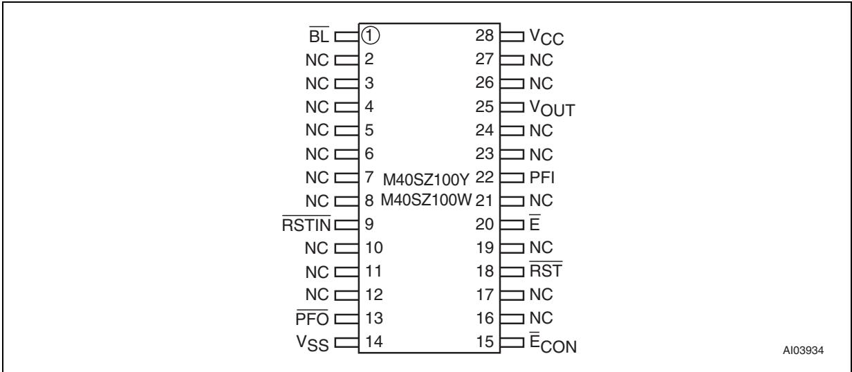
Figure 3. SOIC28 connections
