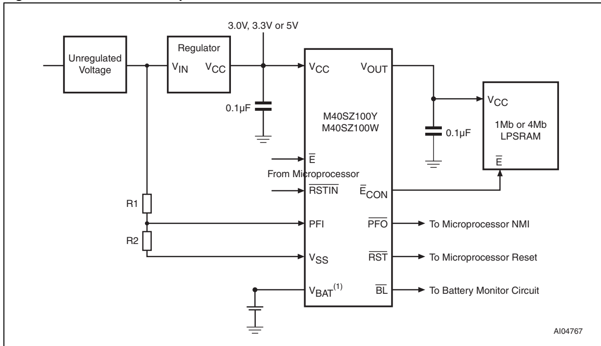
Figure 5. Hardware hookup
