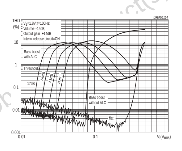
Figure 13. BASS ALC: THD
