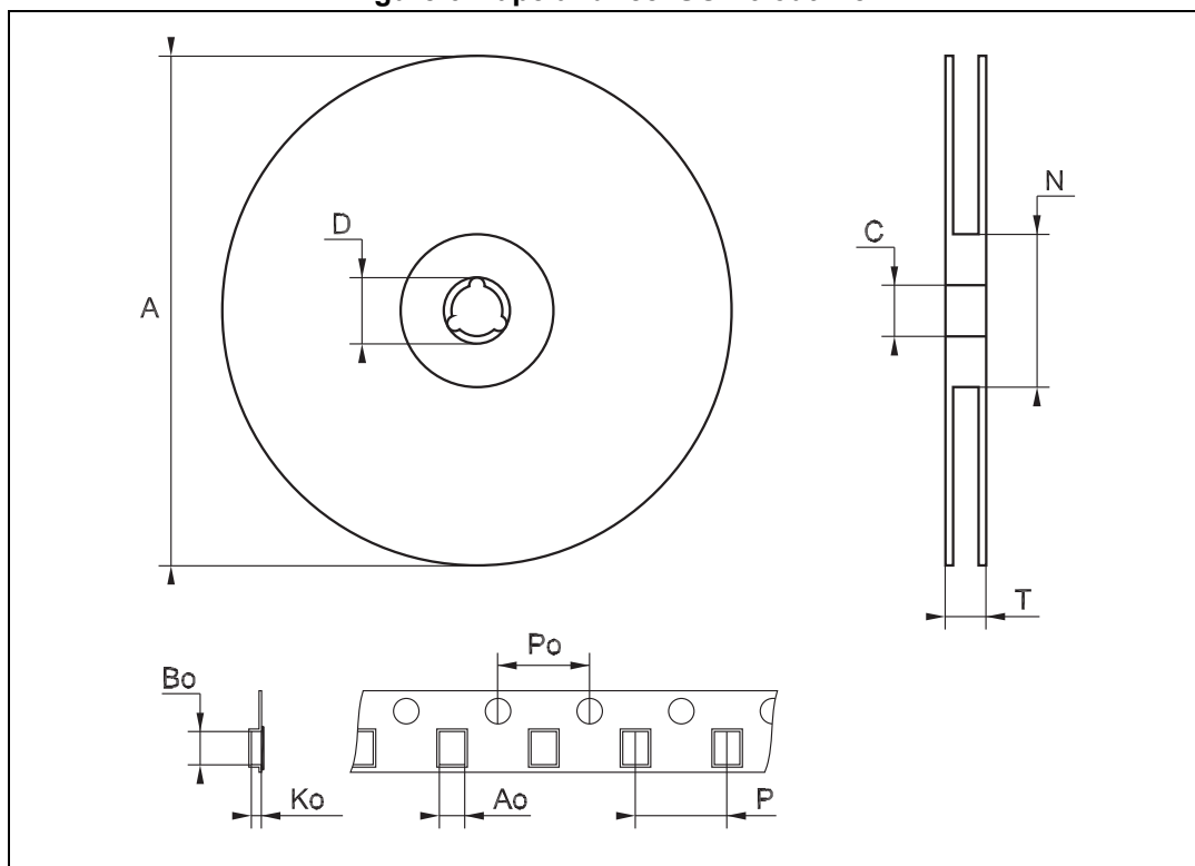
Figure 6. Tape and reel SO-16 outline
