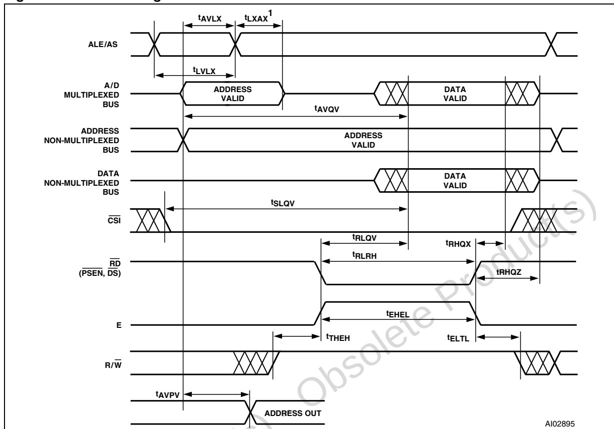
Figure 44. READ timing
