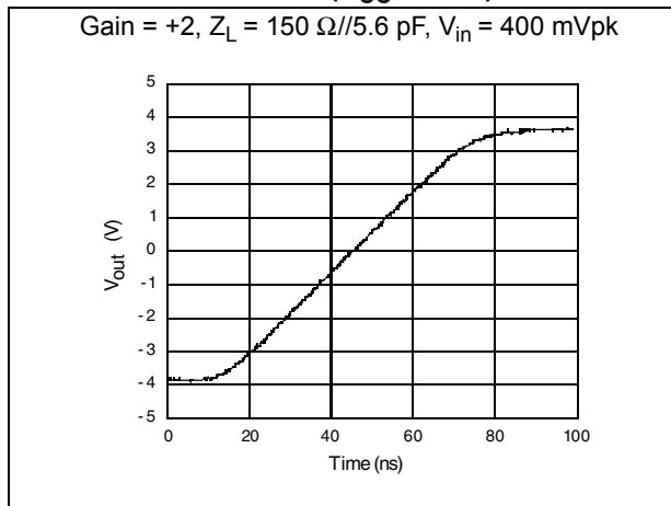
Figure 21. Large signal measurement - positive slew rate ( V_{CC} = \pm 5\text{ V} )
