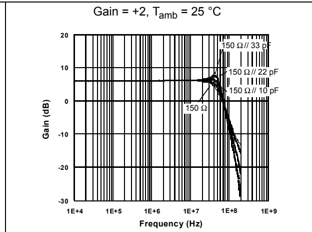
Figure 18. Overshoot vs. output capacitance ( V_{CC} = \pm 5\text{ V} )
