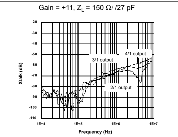
Figure 26. Channel separation (crosstalk) vs. frequency ( V_{CC} = \pm 5\text{ V} )
