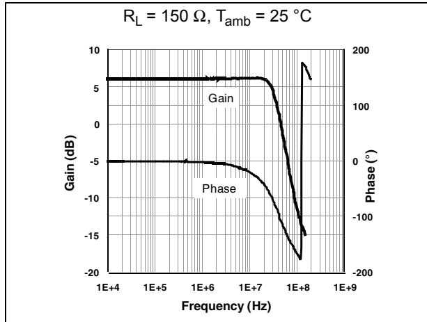
Figure 17. Closed loop gain and phase vs. frequency (gain = +2, V_{CC} = \pm 5\text{ V} )
