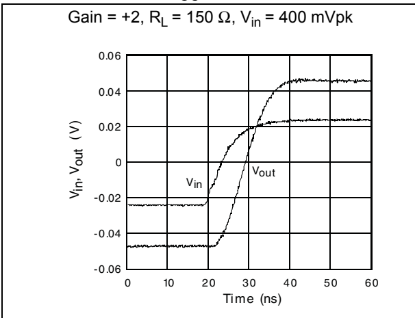
Figure 23. Small signal measurement - rise time ( V_{CC} = \pm 5\text{ V} )
