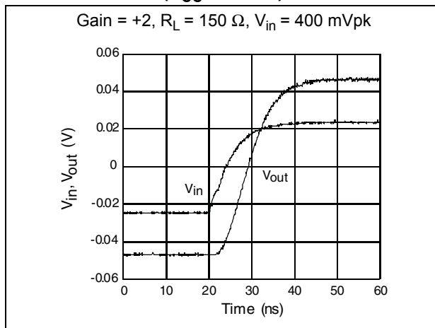
Figure 8. Small signal measurement – rise time ( V_{CC} = \pm 2.5\text{ V} )
