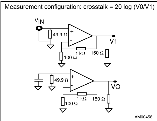
Figure 25. Channel separation (crosstalk) vs. frequency schematic ( V_{CC} = \pm 5\text{ V} )
