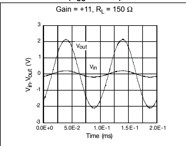
Figure 13. Maximum output swing ( V_{CC} = \pm 2.5\text{ V} )
