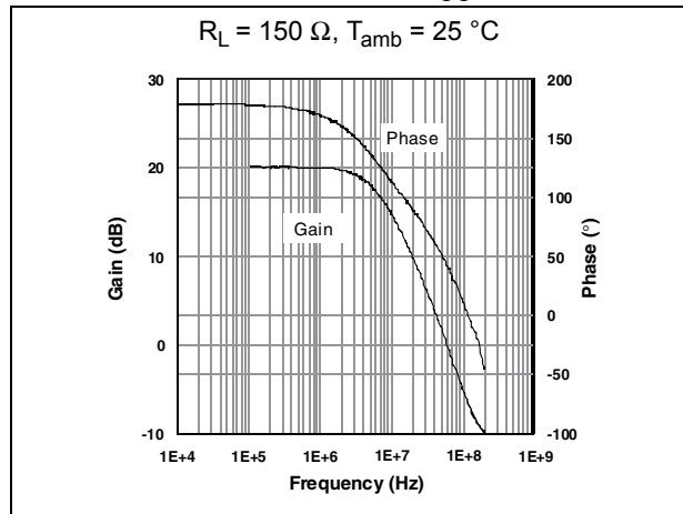
Figure 4. Closed loop gain and phase vs. frequency (gain = -10, V_{CC} = \pm 2.5 V)
