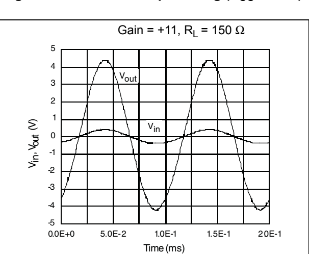
Figure 28. Maximum output swing ( V_{CC} = \pm 5\text{ V} )
