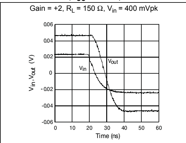
Figure 9. Small signal measurement – fall time ( V_{CC} = \pm 2.5\text{ V} )
