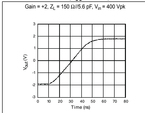
Figure 6. Large signal measurement – positive slew rate ( V_{CC} = \pm 2.5 V)
