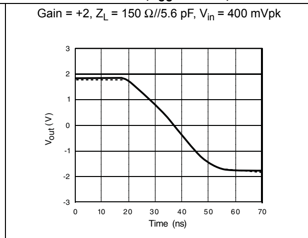
Figure 7. Large signal measurement – negative slew rate ( V_{CC} = \pm 2.5 V)
