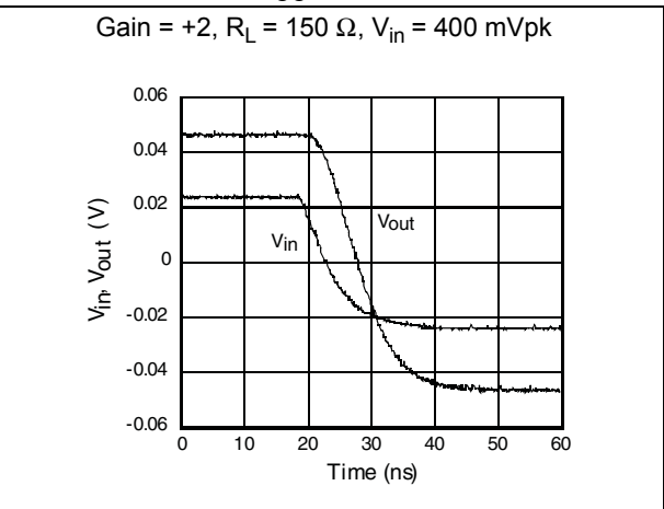
Figure 24. Small signal measurement - fall time ( V_{CC} = \pm 5\text{ V} )
