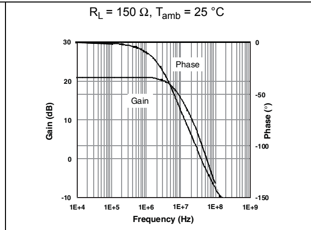
Figure 20. Closed loop gain and phase vs. frequency (gain = +11, V_{CC} = \pm 5\text{ V} )
