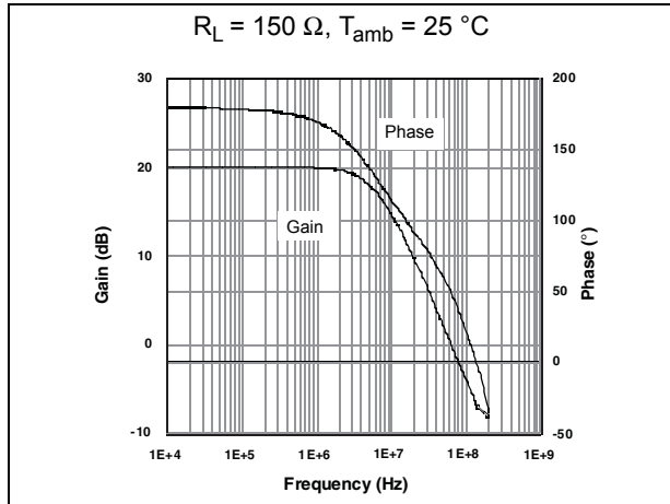
Figure 19. Closed loop gain and phase vs. frequency (gain = -10, V_{CC} = \pm 5\text{ V} )
