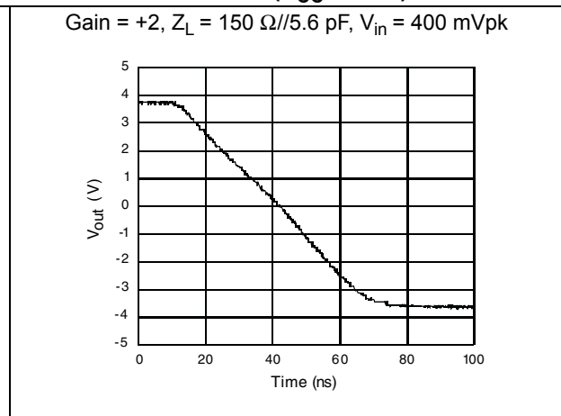
Figure 22. Large signal measurement - negative slew rate ( V_{CC} = \pm 5\text{ V} )
