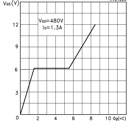
Figure 14: Gate Charge vs Gate-source Voltage
