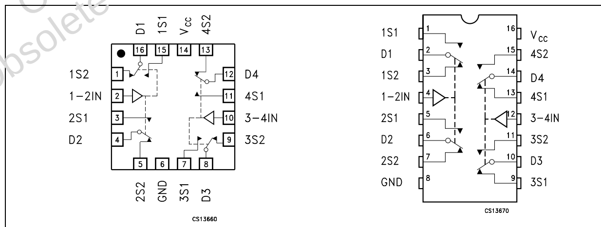
Figure 1: Pin Connection
