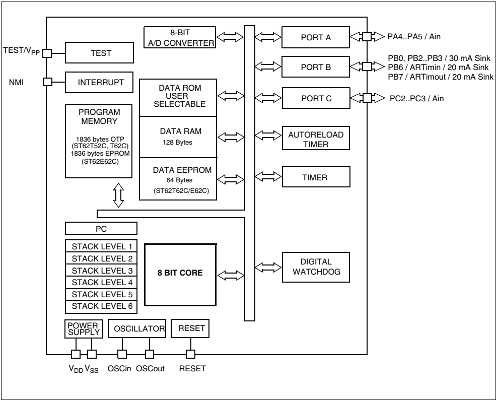
Figure 1. Block Diagram
