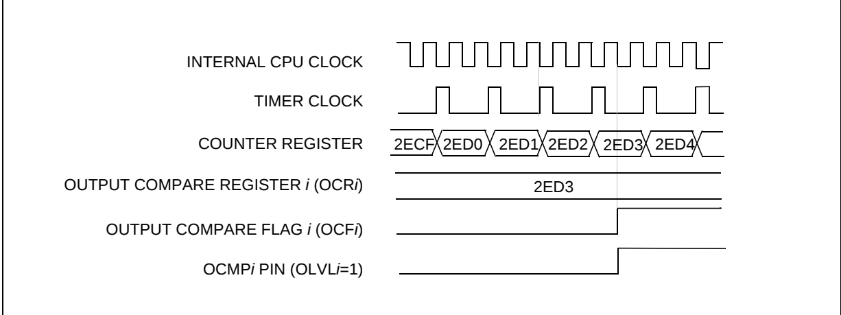
Figure 49. Output Compare Timing Diagram, f_{\text{TIMER}} = f_{\text{CPU}}/2
