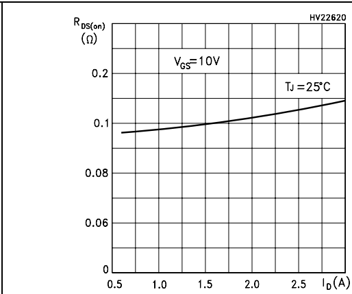
Figure 18. Static drain-source on resistance p-ch
