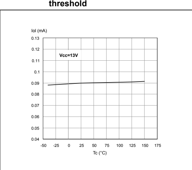
Figure 22. Openload on-state detection threshold
