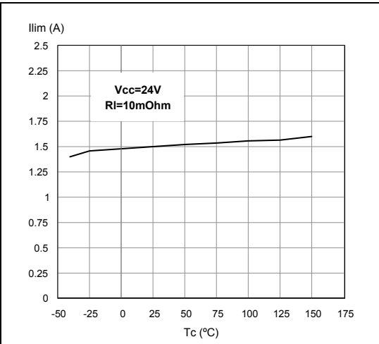
Figure 20. I_{LIM} vs T_{case}
